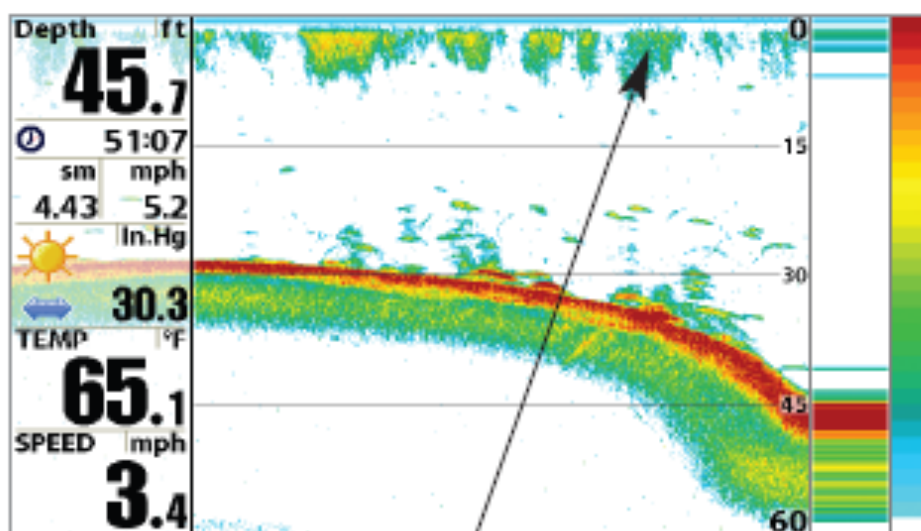
Surface Clutter
