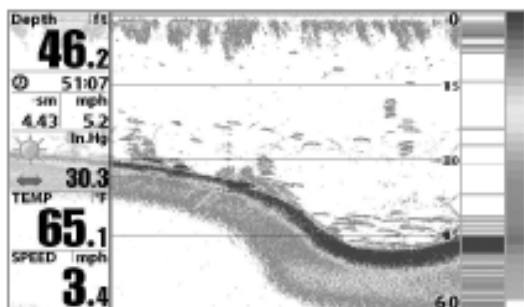
RTS® Window (Narrow)
